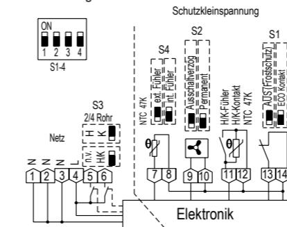
Circuit diagram KTRRB-117.169
