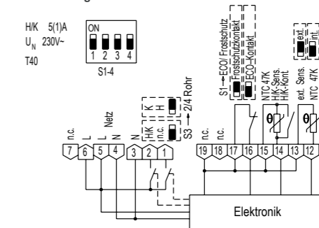
Circuit diagram KTRRB-117.163
