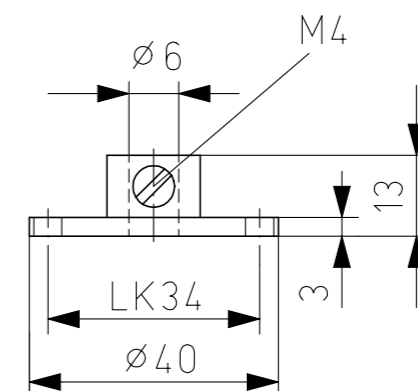
Mounting flange MF
